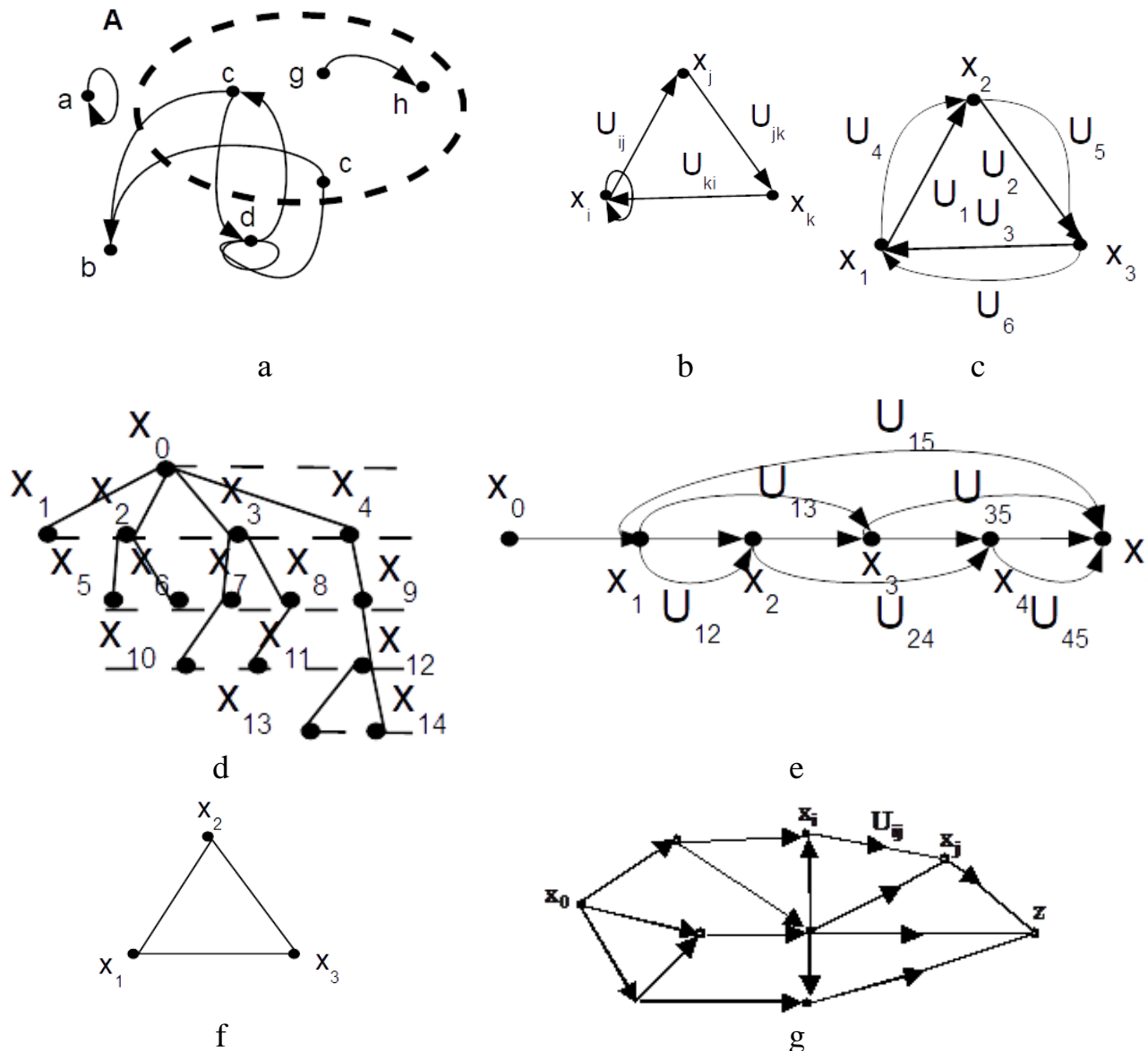
Fig. 1. Examples of graph models:
