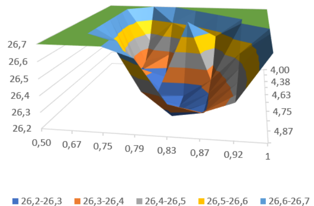
Fig. 7. The minimization results surface functional for the control signal: a – general view; b – enlarged fragment
