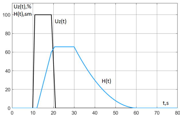
Fig. 4. Results of computer simulation at Uz=100%; t=10 s
