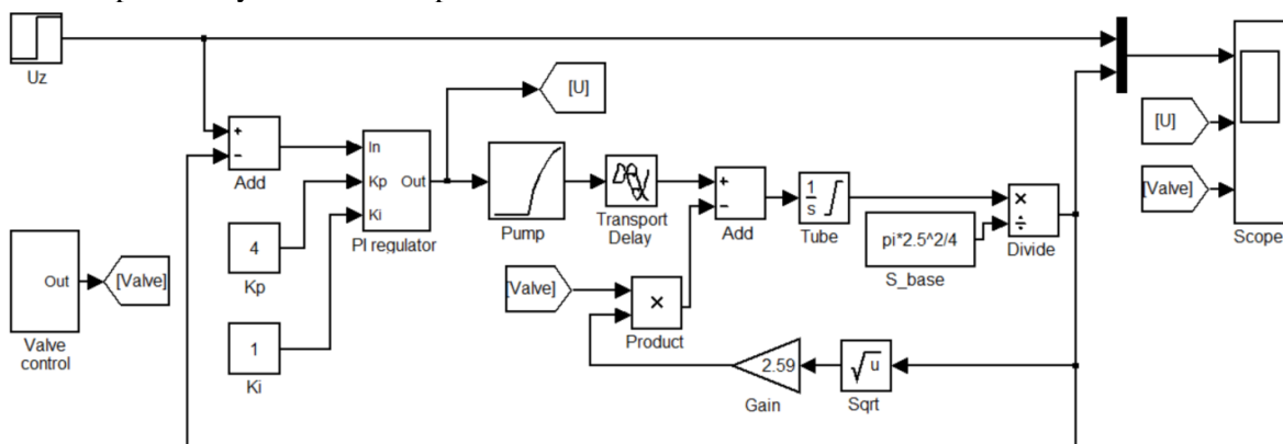
Fig. 6. A modified computer model of the automatic liquid level control system
