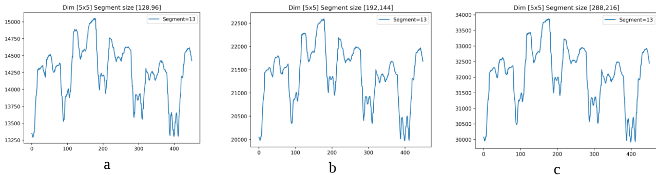
Fig. 10. Segment 13 Ky Fan norm fluctuations for frames divided by 25 blocks (a) 640x480, (b) 960x720 (c) 1440x1080
