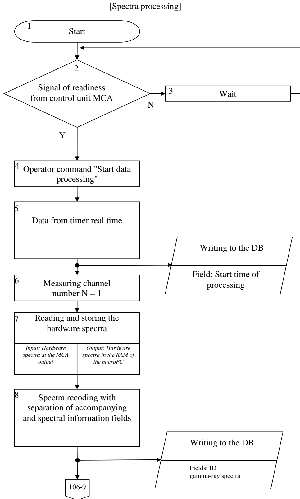
Fig. 5a. Gamma-ray spectra processing. Part 1
