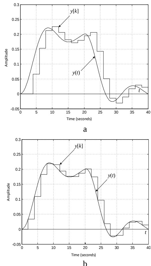
Fig. 5. The response of a continuous system and its discrete analogues, determined by the method of zero of poles matching at m_d = n-1 (a) and m_d = n (b) on the linear input signal
