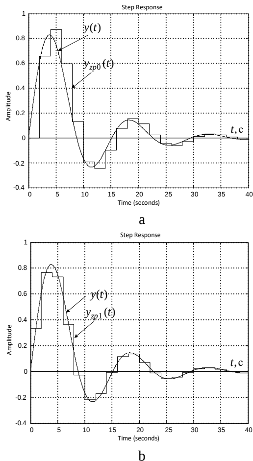
Fig. 4. Step response of a continuous system and its discrete analogues, determined by the method of zero of poles matching at m_d = n-1 (a) and m_d = n (b)
